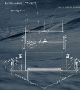
SECTION G-G
