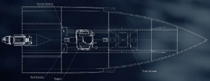
SECTION B-B Below deck
